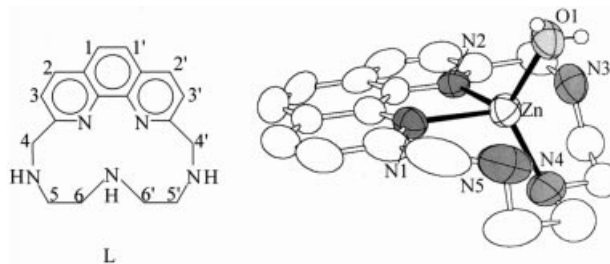
Figure 1. L drawing (with atom labelling used in NMR spectroscopic experiments) and crystal structure of the [ZnL(H 2 O)] 2+ cation.
