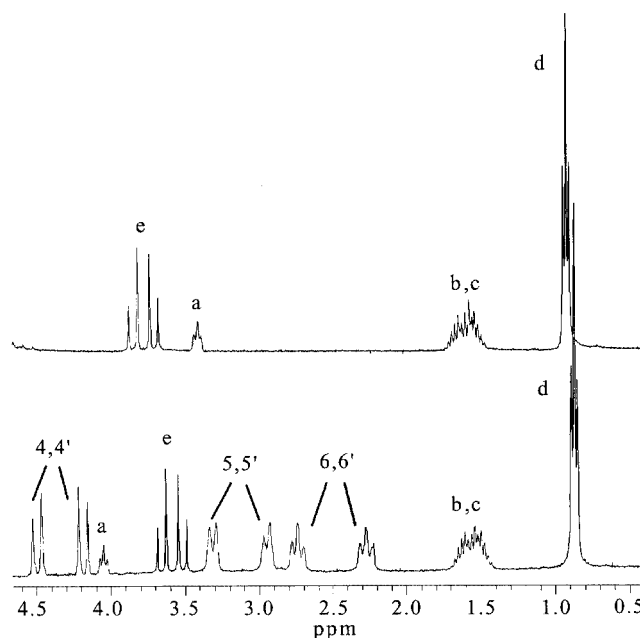
Figure 5. ^1\text{H} NMR spectra of Leu-Gly ^- (a) and [\text{ZnL}(\text{Leu-Gly})]^+ (pH, 8.5) (b). (See Scheme 1 and Figure 1 for the labelling used).
