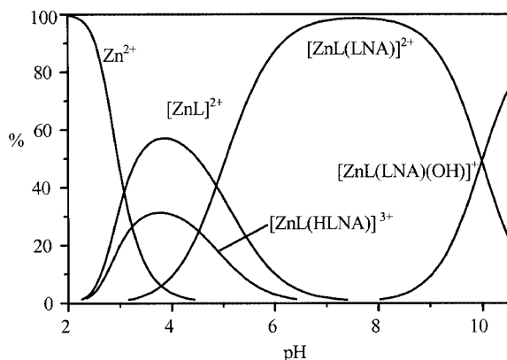
Figure 6. Species distribution diagram for the system [\text{ZnL}]^{2+}/\text{LNA} in 1:1 molar ratio ( \text{NMe}_4\text{NO}_3 0.1 M, 308.1 K).
