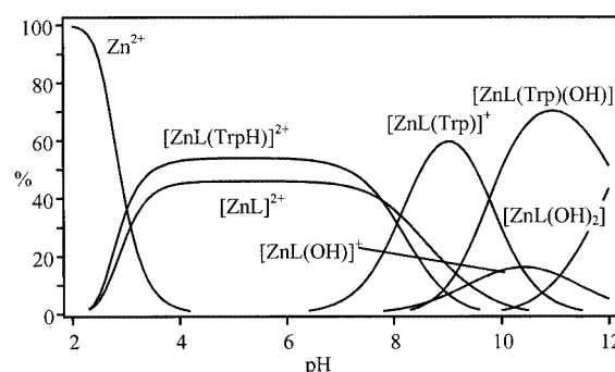
Figure 3. Species distribution diagram for the system [\text{ZnL}]^{2+}/\text{Trp} in 1:1 molar ratio ( \text{NMe}_4\text{NO}_3 0.1 M, 298 K).
