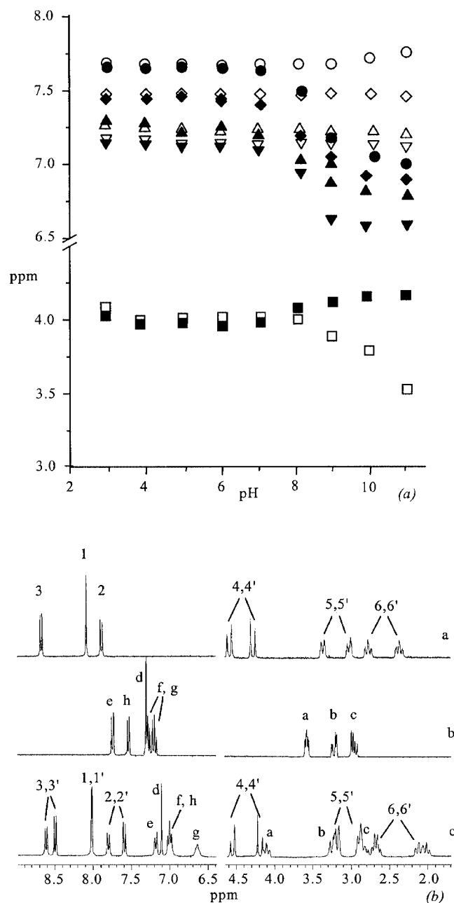
Figure 4. (a): pH dependence of the 1 H NMR chemical shifts of selected protons of Trp in the absence (□: a proton; ▽: g; △: f; ◇: h; ○: e), and in the presence of the Zn II complex with L (■: a proton; ▼: g; ▲: h; ●: e). The signals of the protons b, c and d are omitted for clarity. (b): 1 H NMR spectra of [ZnL] 2+ (a), Trp - (b) and [ZnL(Trp)] + (pH, 9.3) (c). See Scheme 1 and Figure 1 for the labelling used.
