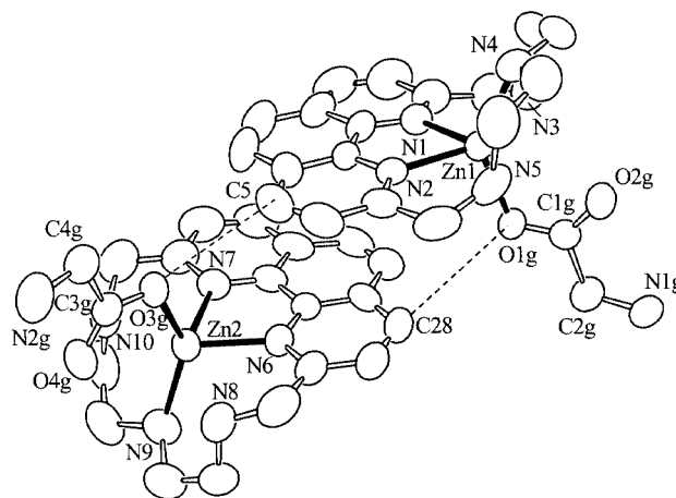
Figure 2. ORTEP drawing of the [ZnL(HGly)] 2+ complex, representing the A and B independent units coupled by \pi -stacking and C–H···O hydrogen bond interactions
